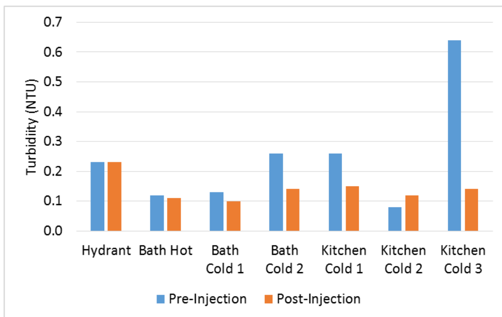
Figure 6. Turbidity data for Home A.
