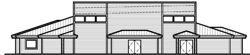
Schematic NORTH ELEVATION 1/16" = 1'-0"
