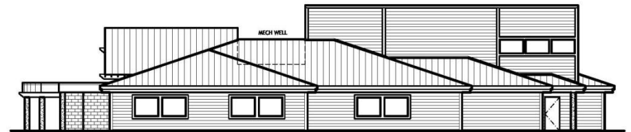
Schematic EAST ELEVATION 1/16" = 1'-0"
